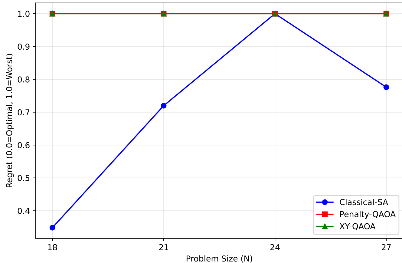
Normalized Regret vs N (BB2, Train N=200)
