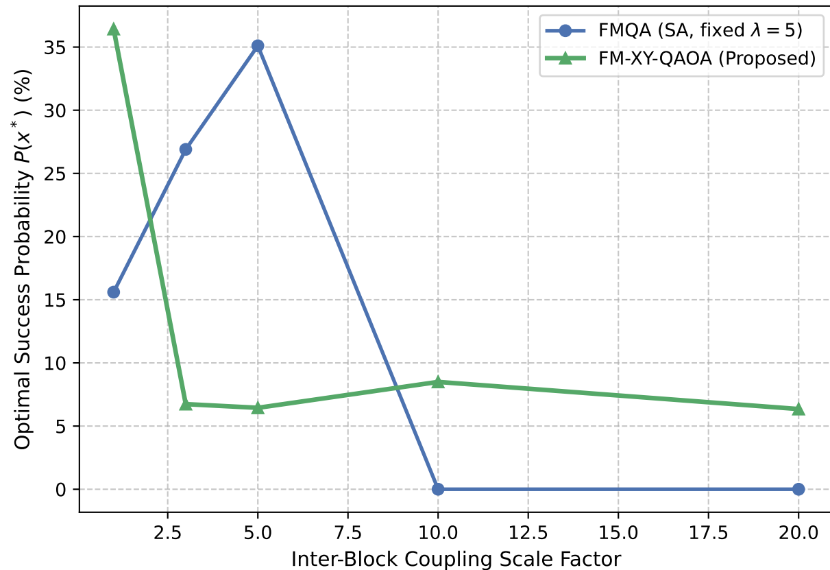
Success Rate under Heterogeneous Scales
