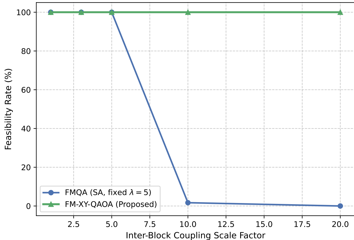
Constraint Robustness vs Scale Discrepancy
