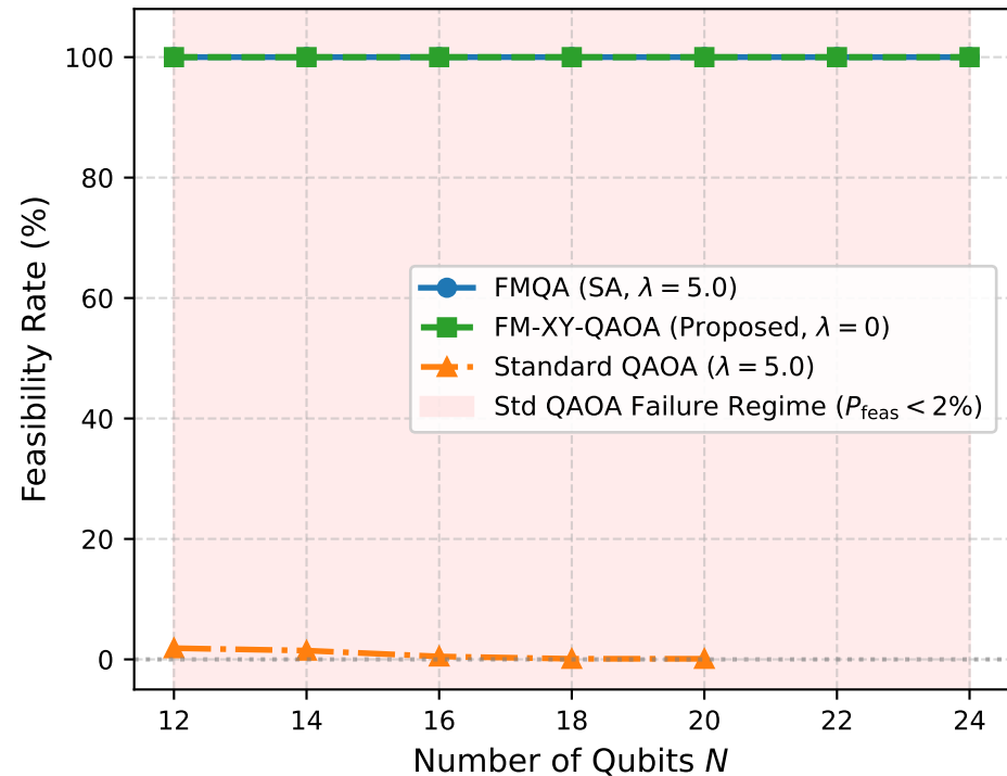
(a) Feasibility Collapse vs Perfect Preservation
