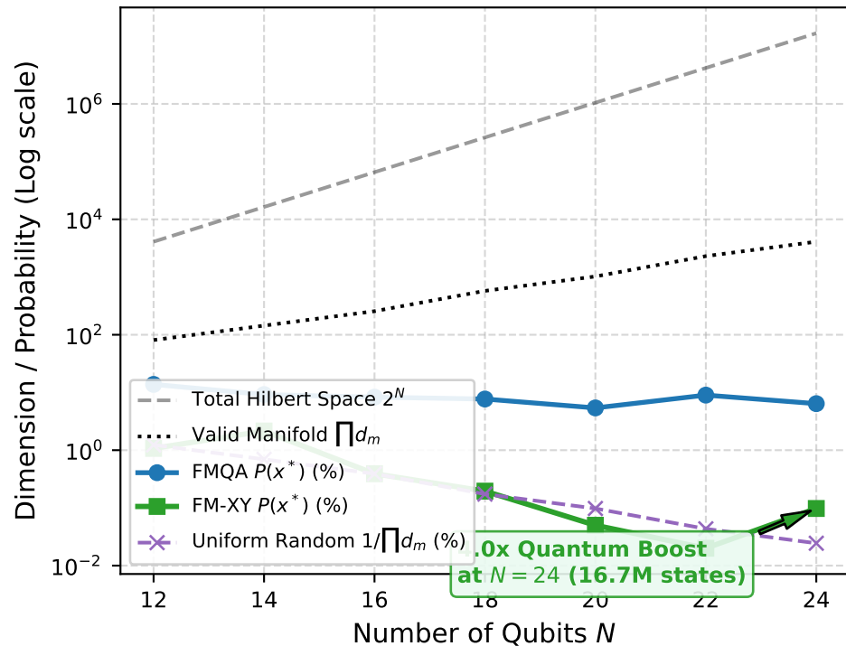
(b) State Sparsity & Extreme Scaling ( N \leq 24 )
