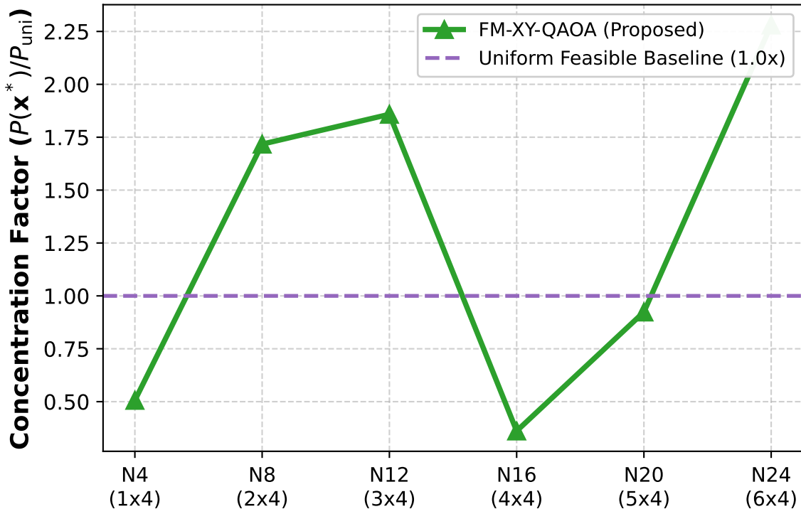
(a) Quantum Concentration Advantage
