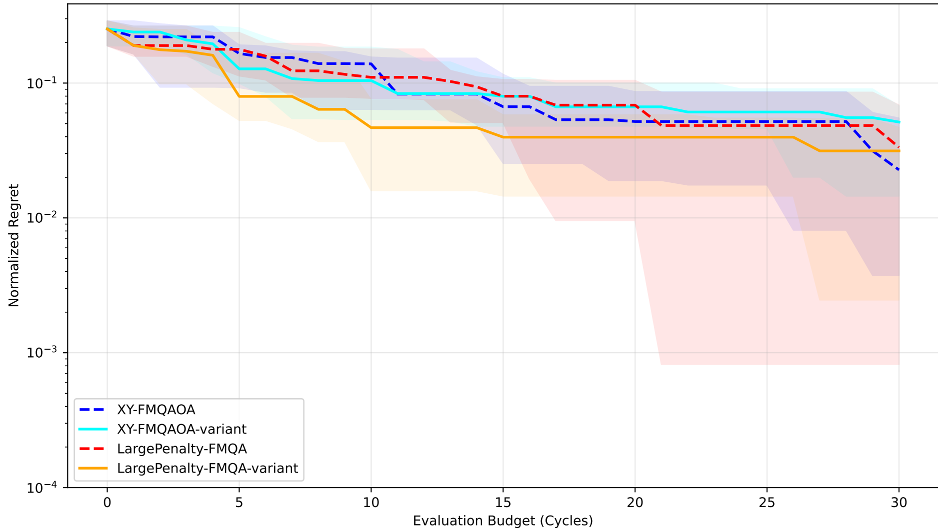
Median Convergence: BB1 N=24 (10 seeds)
