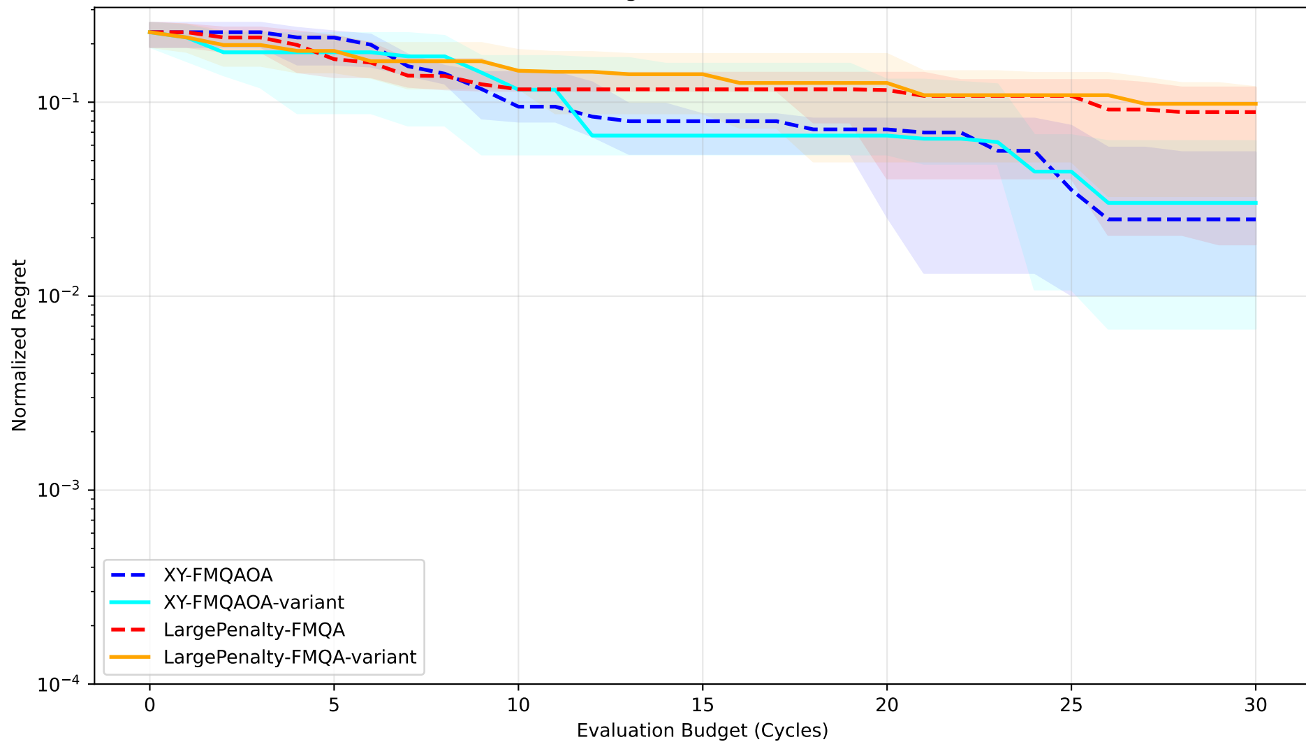
Median Convergence: BB1 N=27 (10 seeds)
