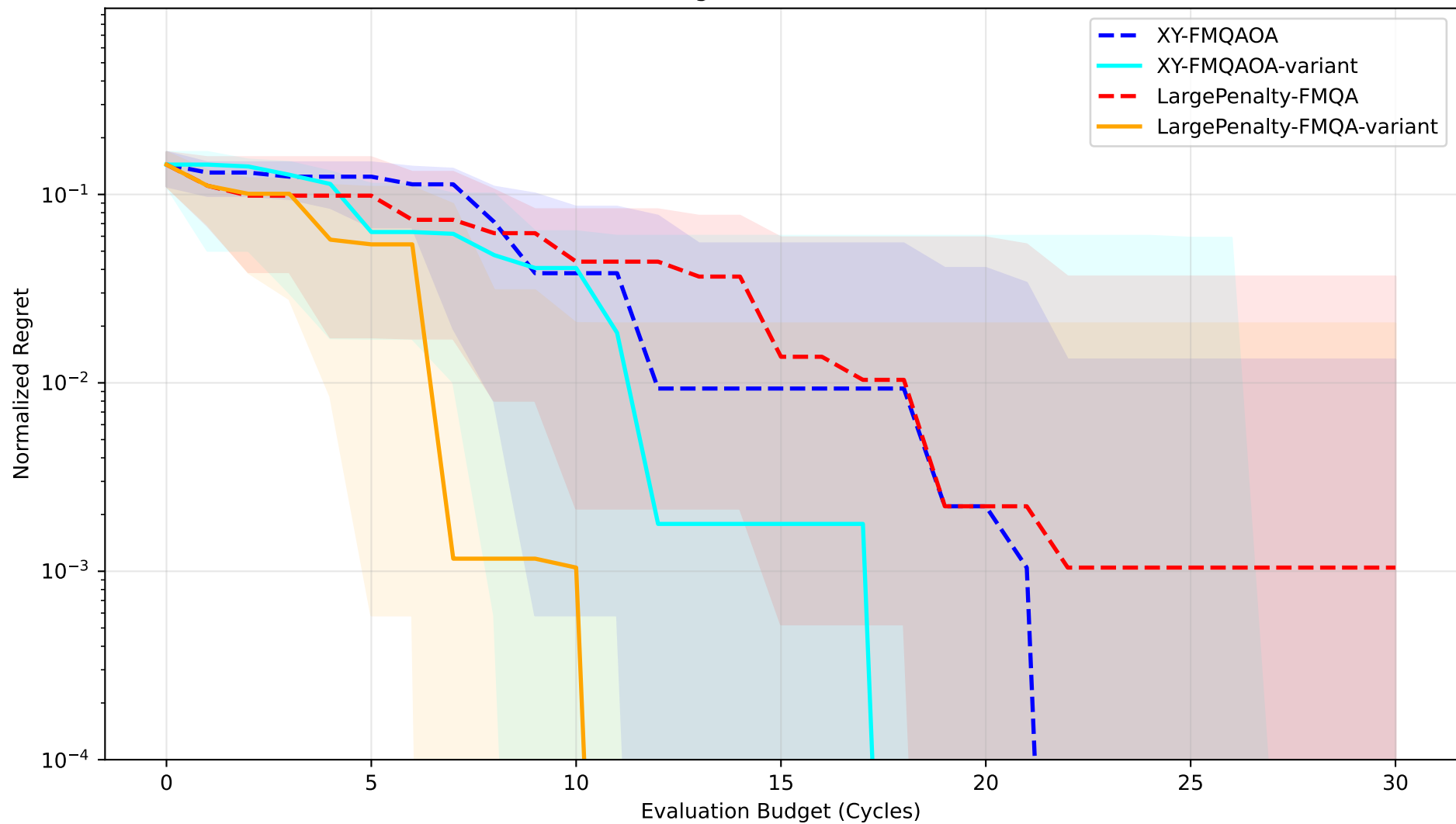
Median Convergence: BB2 N=21 (10 seeds)
