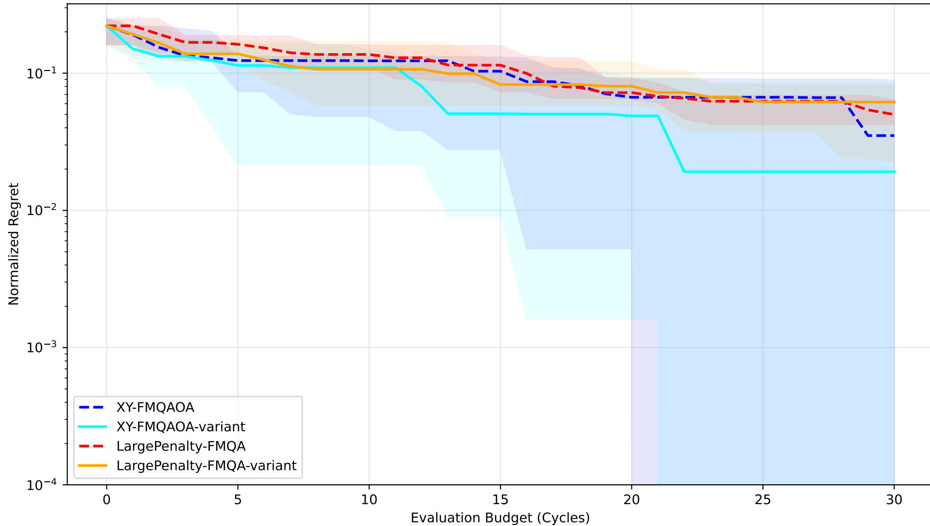
Median Convergence: BB2 N=27 (10 seeds)
