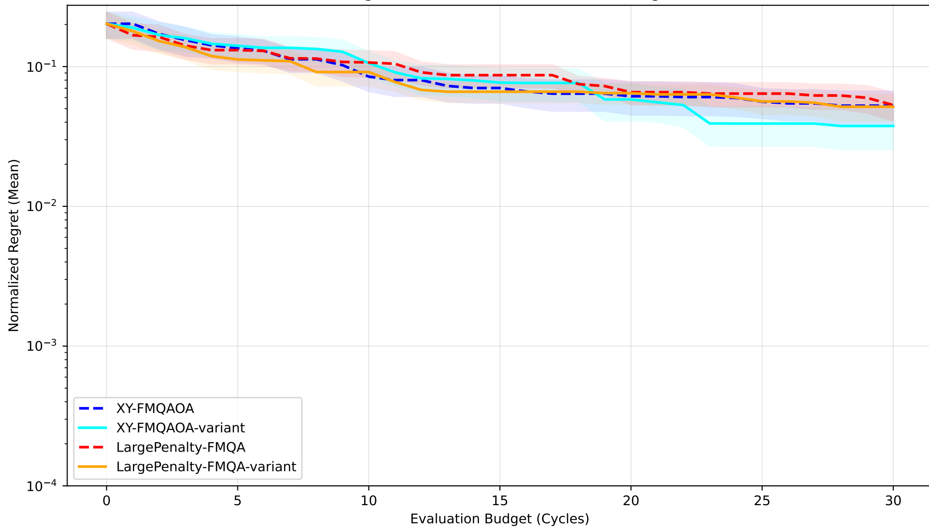
Mean Convergence: BB1 N=21 (10 seeds, shading: +/- SEM)
