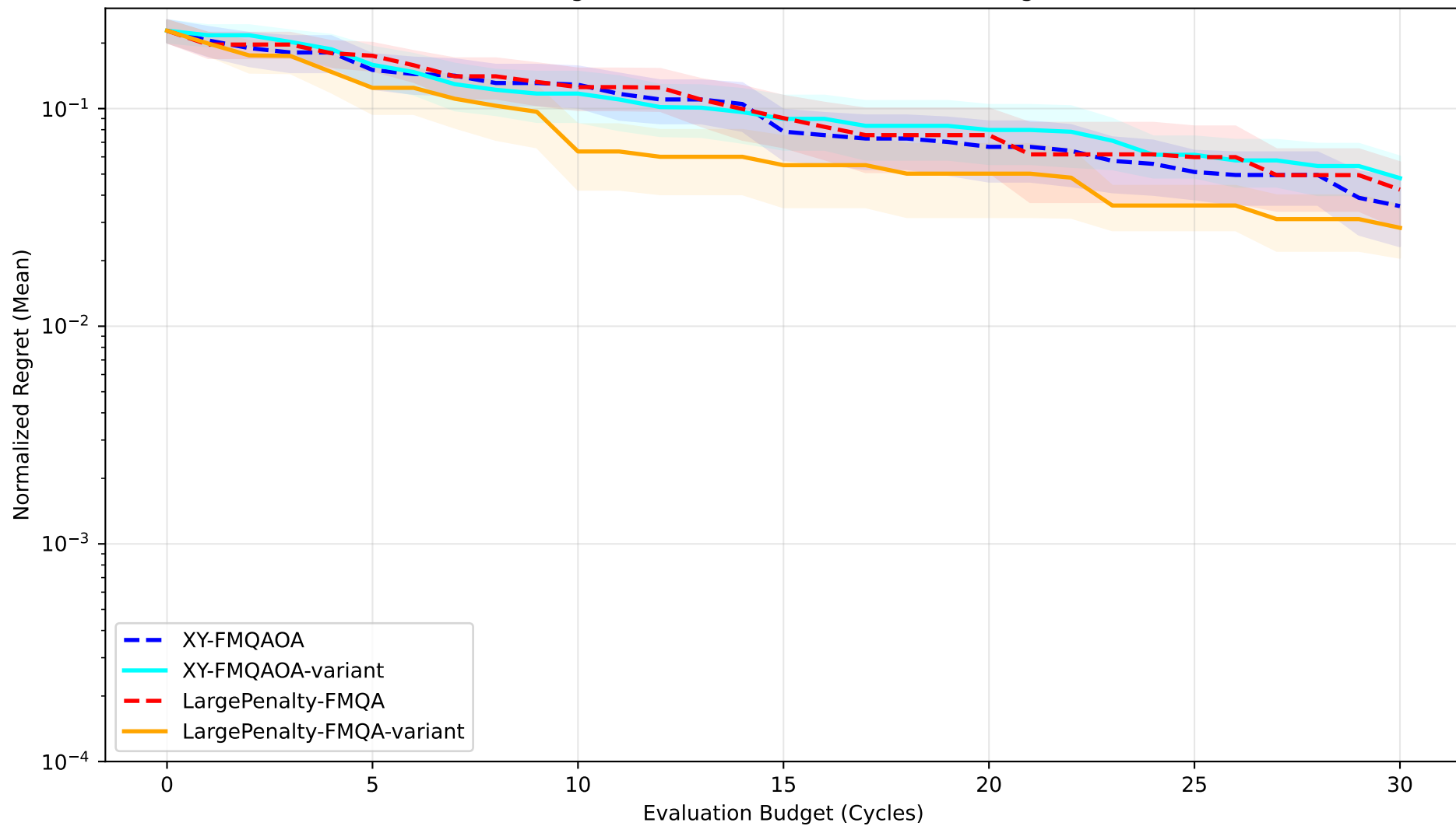
Mean Convergence: BB1 N=24 (10 seeds, shading: +/- SEM)
