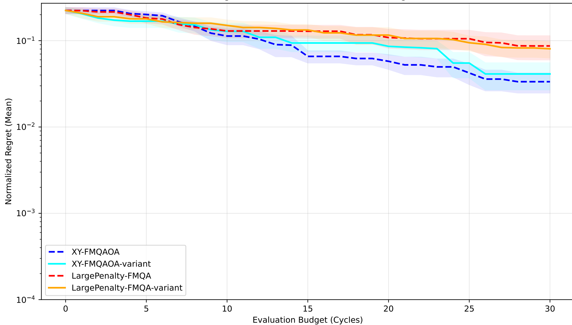
Mean Convergence: BB1 N=27 (10 seeds, shading: +/- SEM)
