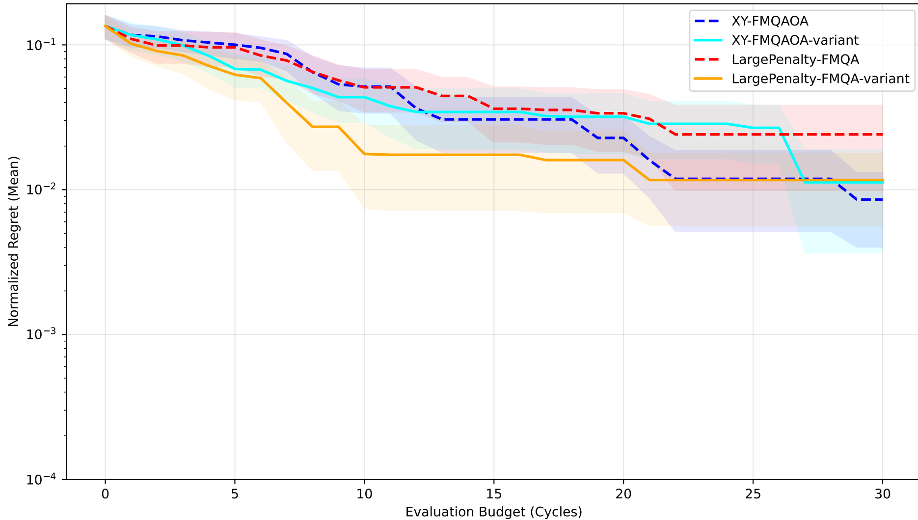
Mean Convergence: BB2 N=21 (10 seeds, shading: +/- SEM)
