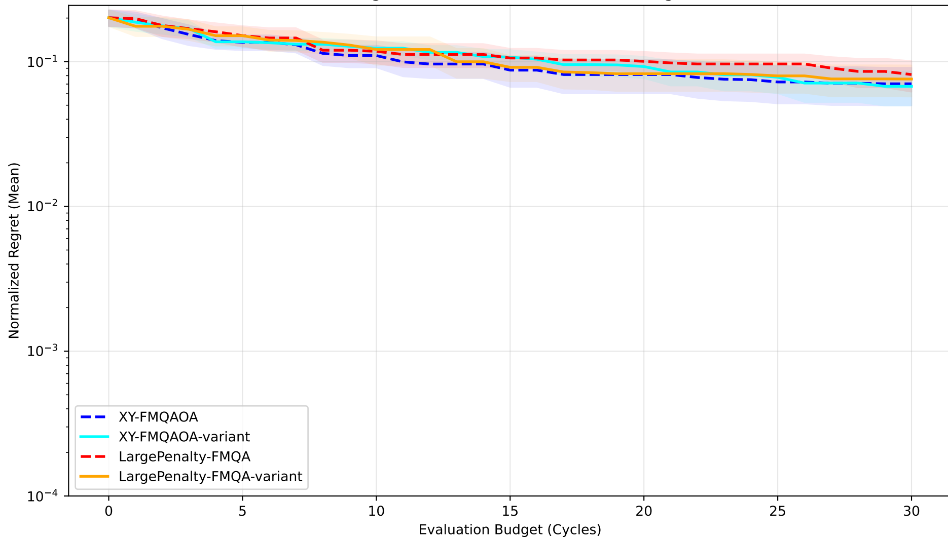
Mean Convergence: BB2 N=24 (10 seeds, shading: +/- SEM)
