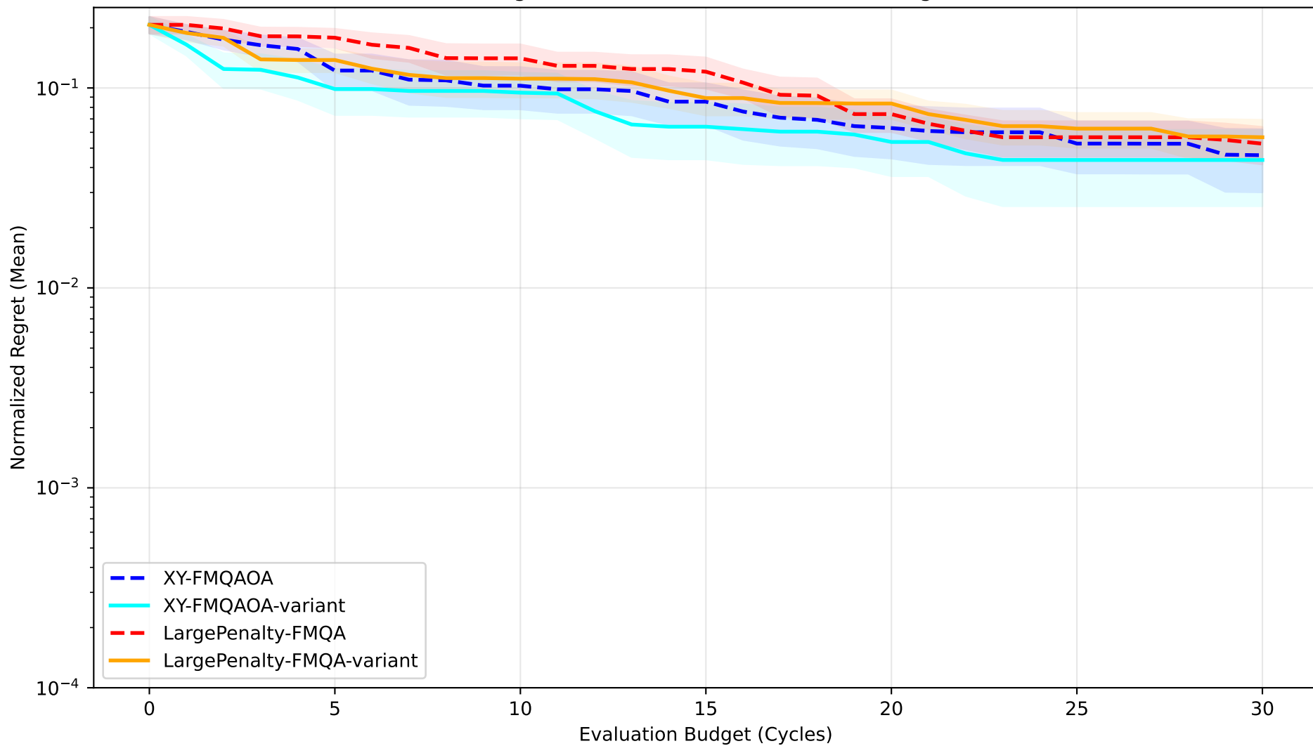
Mean Convergence: BB2 N=27 (10 seeds, shading: +/- SEM)
