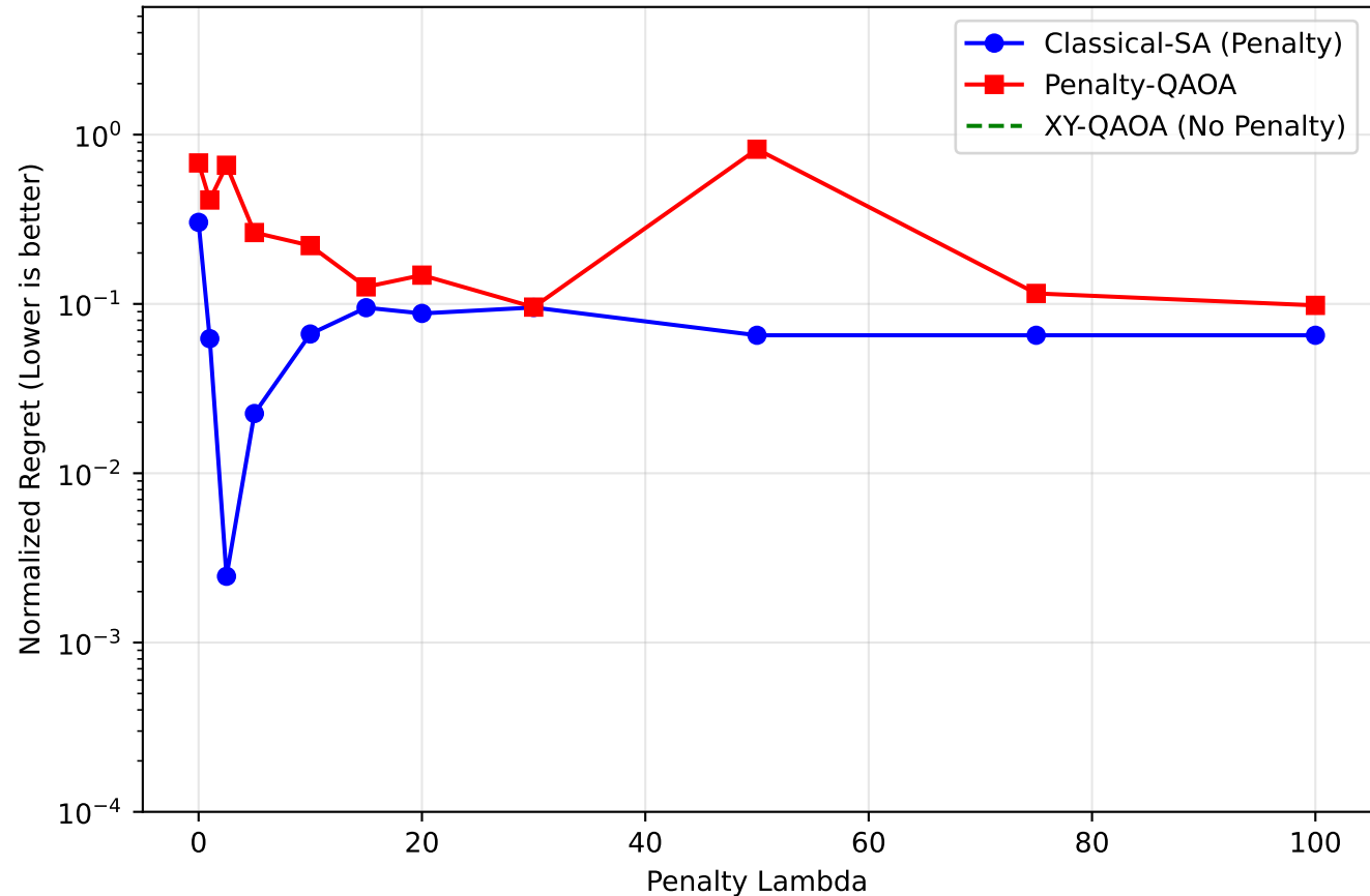
Best Regret vs Lambda (BB2 N=18 (3 seeds mean))
