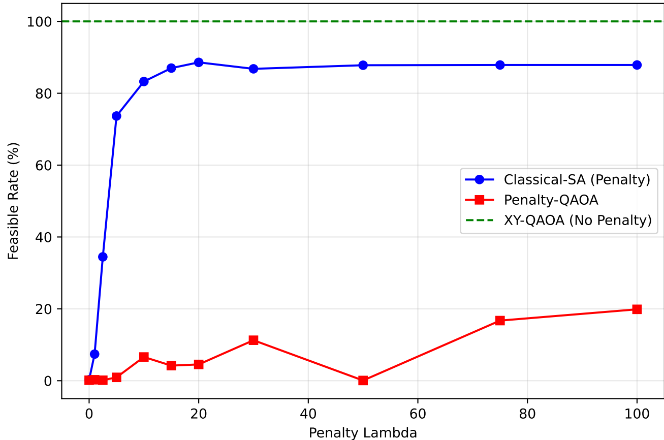
Feasible Rate vs Lambda (BB2 N=18 (3 seeds mean))
