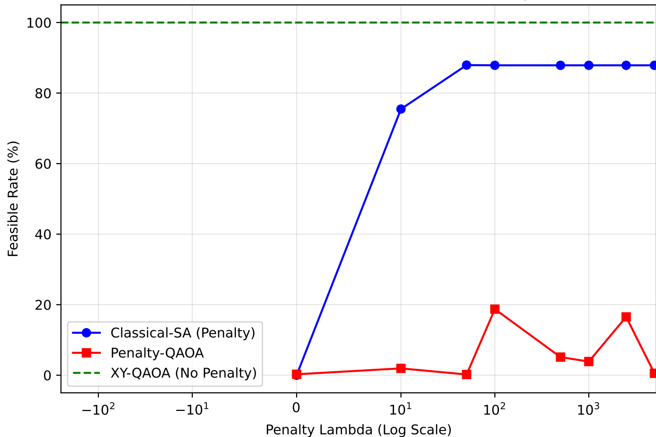
Feasible Rate vs Lambda (BB1 N=18 (3 seeds mean, Up to L=5000))
