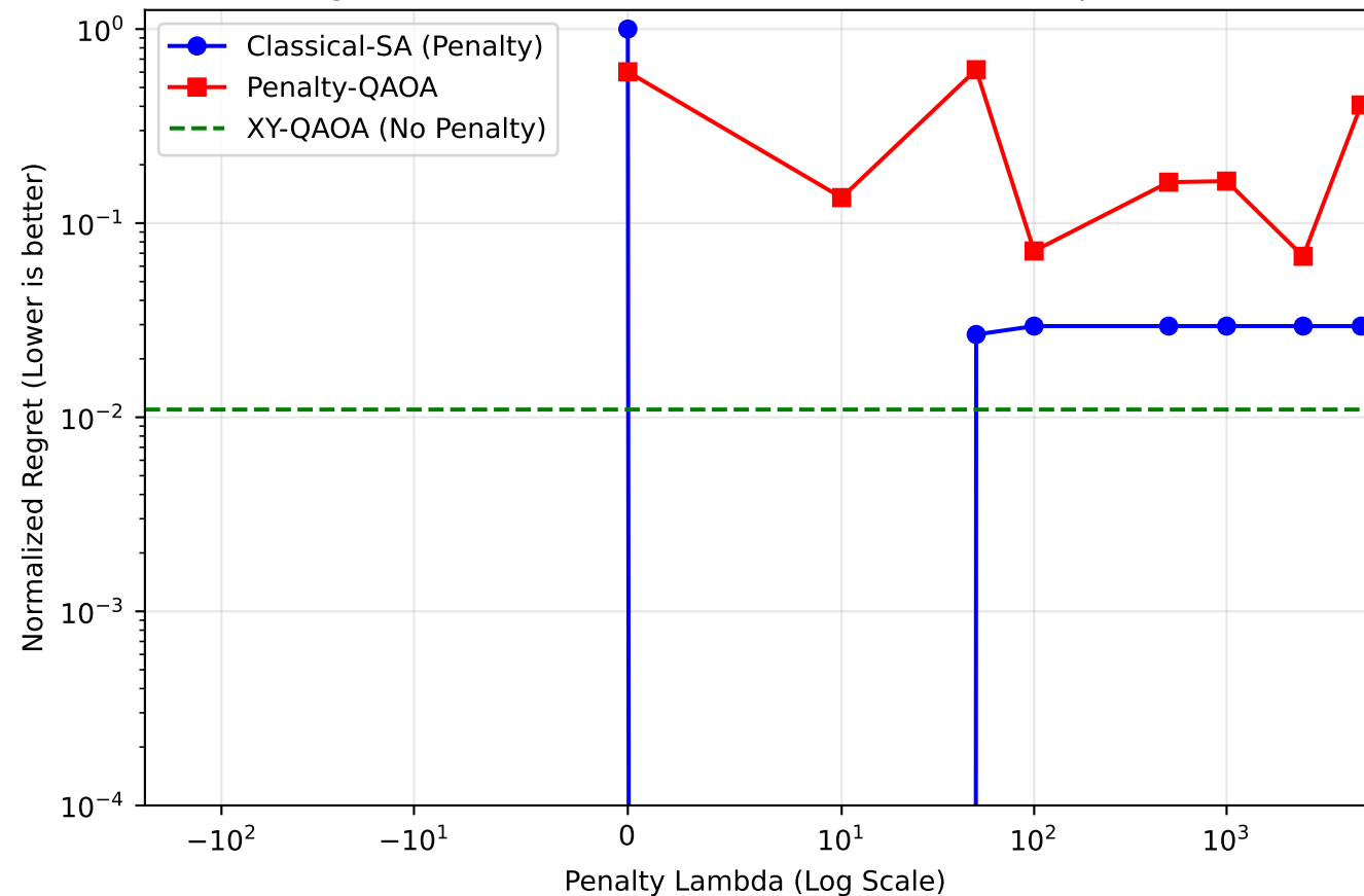
Best Regret vs Lambda (BB1 N=18 (3 seeds mean, Up to L=5000))
