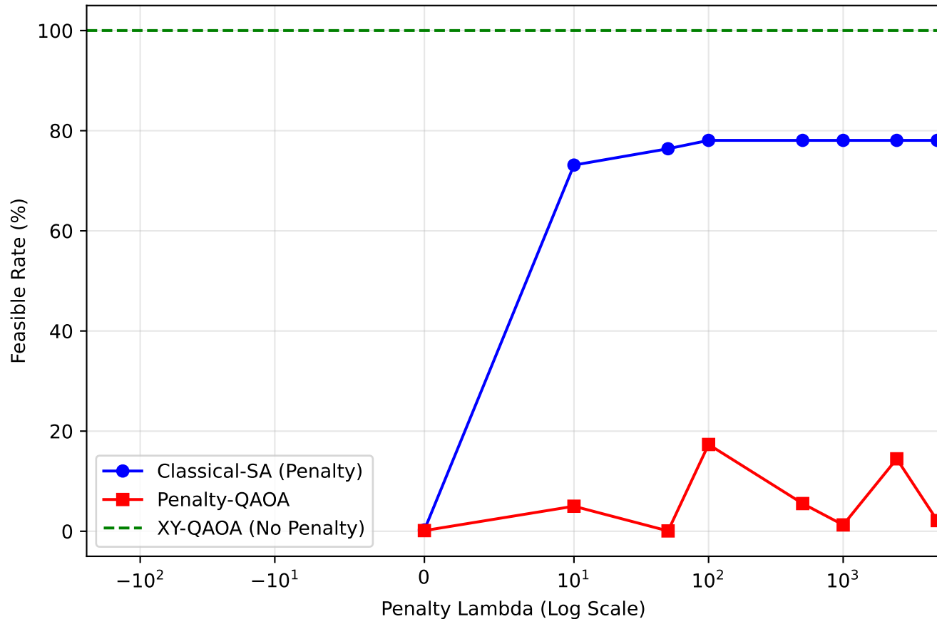
Feasible Rate vs Lambda (BB2 N=21 (3 seeds mean, Up to L=5000))
