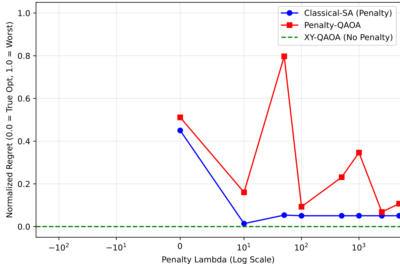
Best Regret vs Lambda (BB2 N=21 (3 seeds mean, Up to L=5000))
