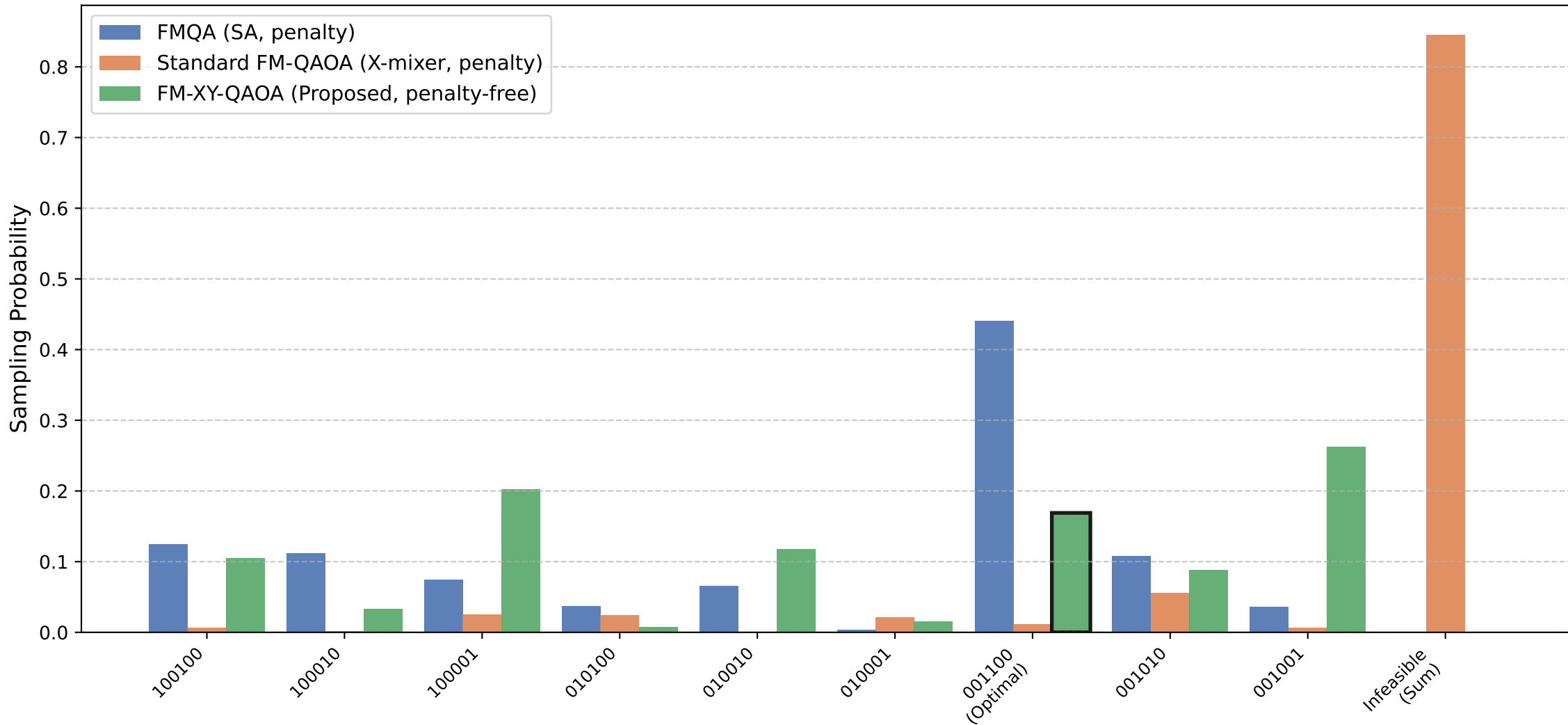
Sampling Probability Distribution Comparison (N=6, blocks=[3, 3], \lambda=5.0 )
