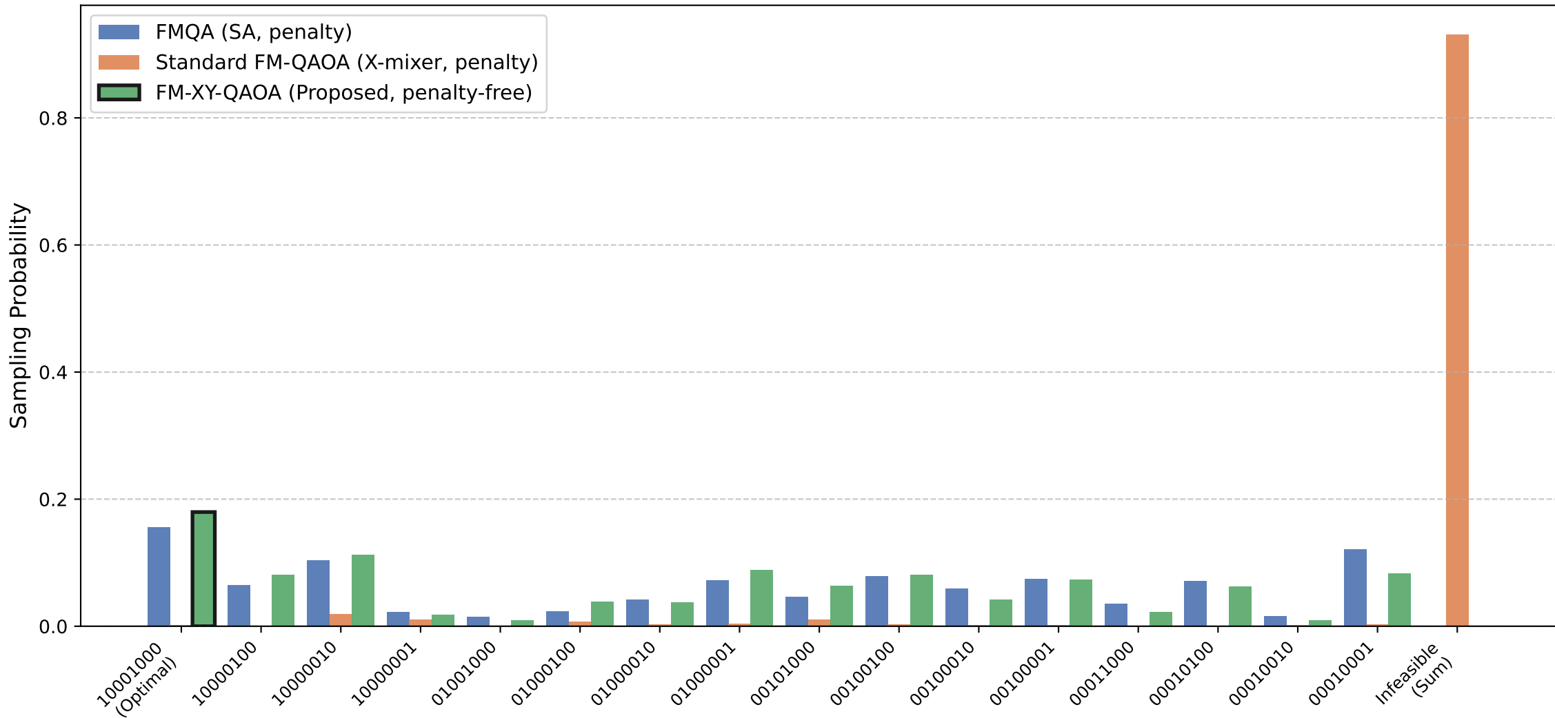
Sampling Probability Distribution Comparison (N=8, blocks=[4, 4], \lambda=5.0 )
