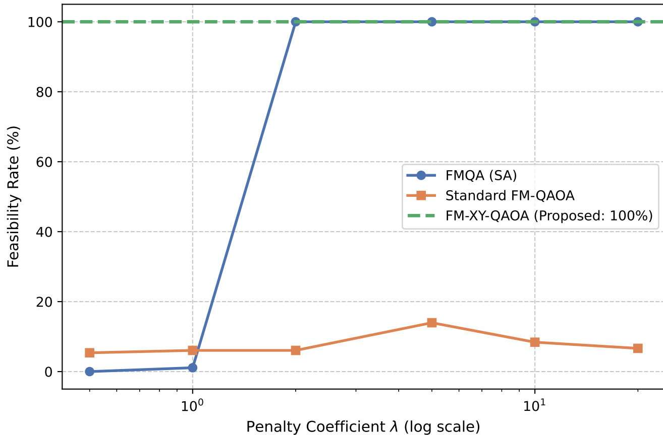
Constraint Feasibility vs Penalty \lambda
