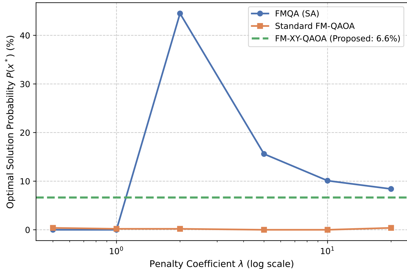
Success Probability P(x^*) vs Penalty \lambda
