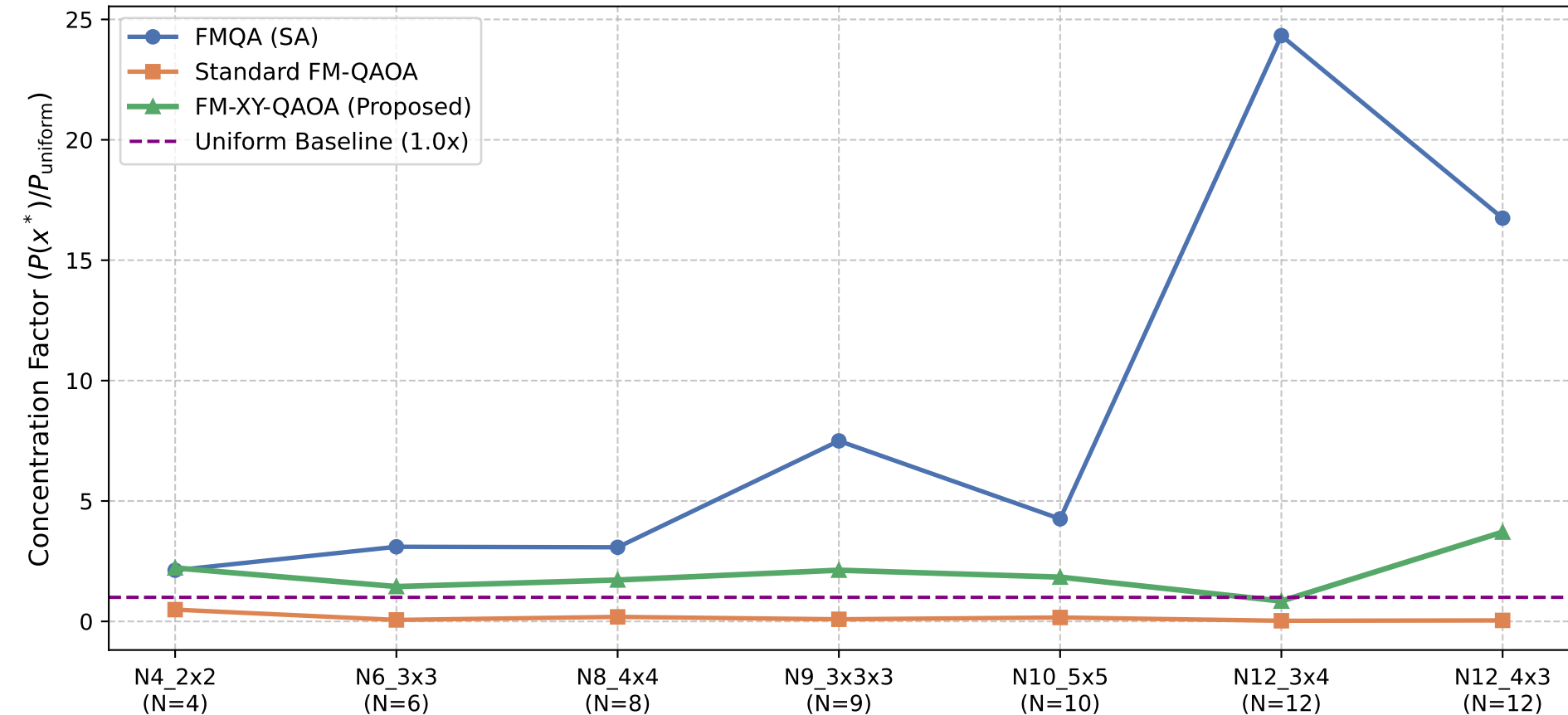
Quantum Optimization Concentration Advantage
