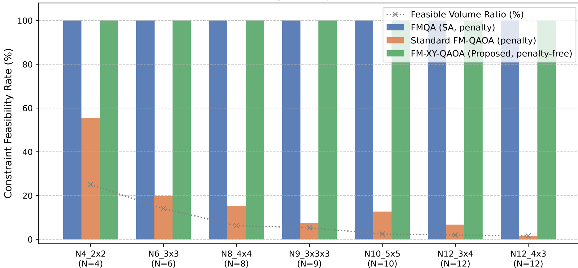
Constraint Feasibility Scaling across Problem Sizes
