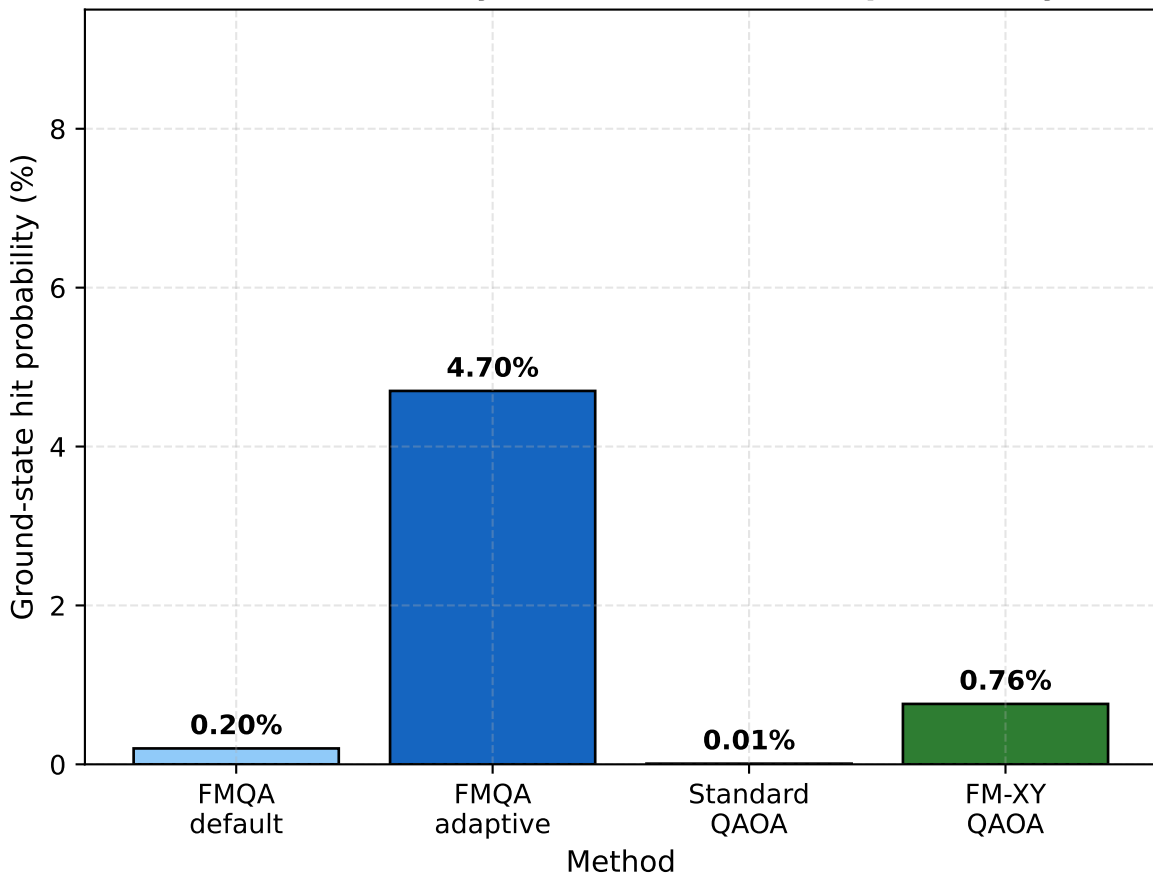
BB-1 Materials Catalyst: Ground-state hit probability (%)
