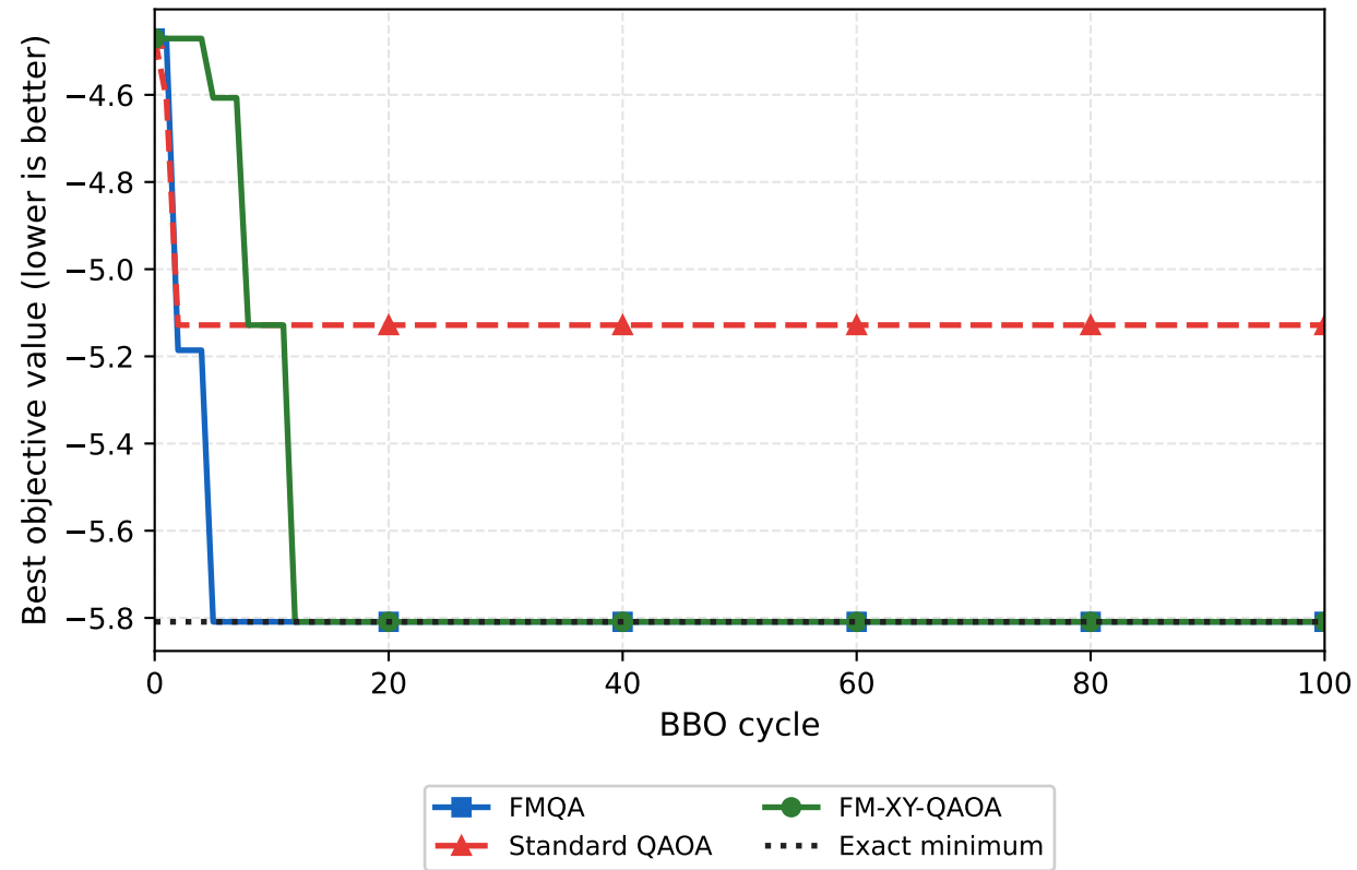
BB-2 Fully-Connected Random: 100-Cycle BBO Trajectory
