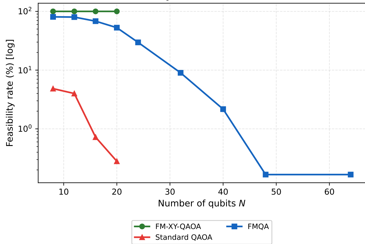
Feasibility vs Number of Qubits
