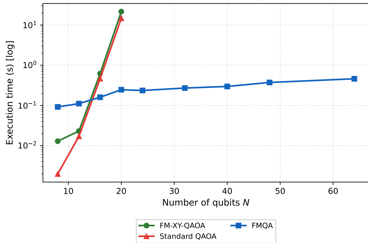
Runtime vs Number of Qubits
