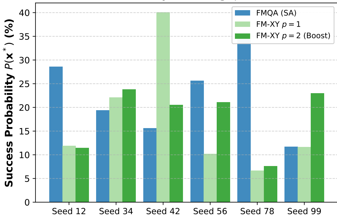
(b) Quantum Layer Scaling ( p = 2 Boost)
