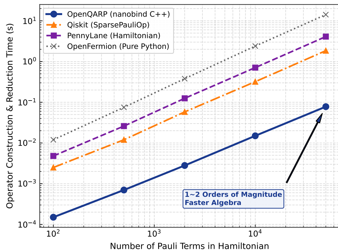
(c) Pauli Operator Algebra Throughput (arXiv:2609.15697)
