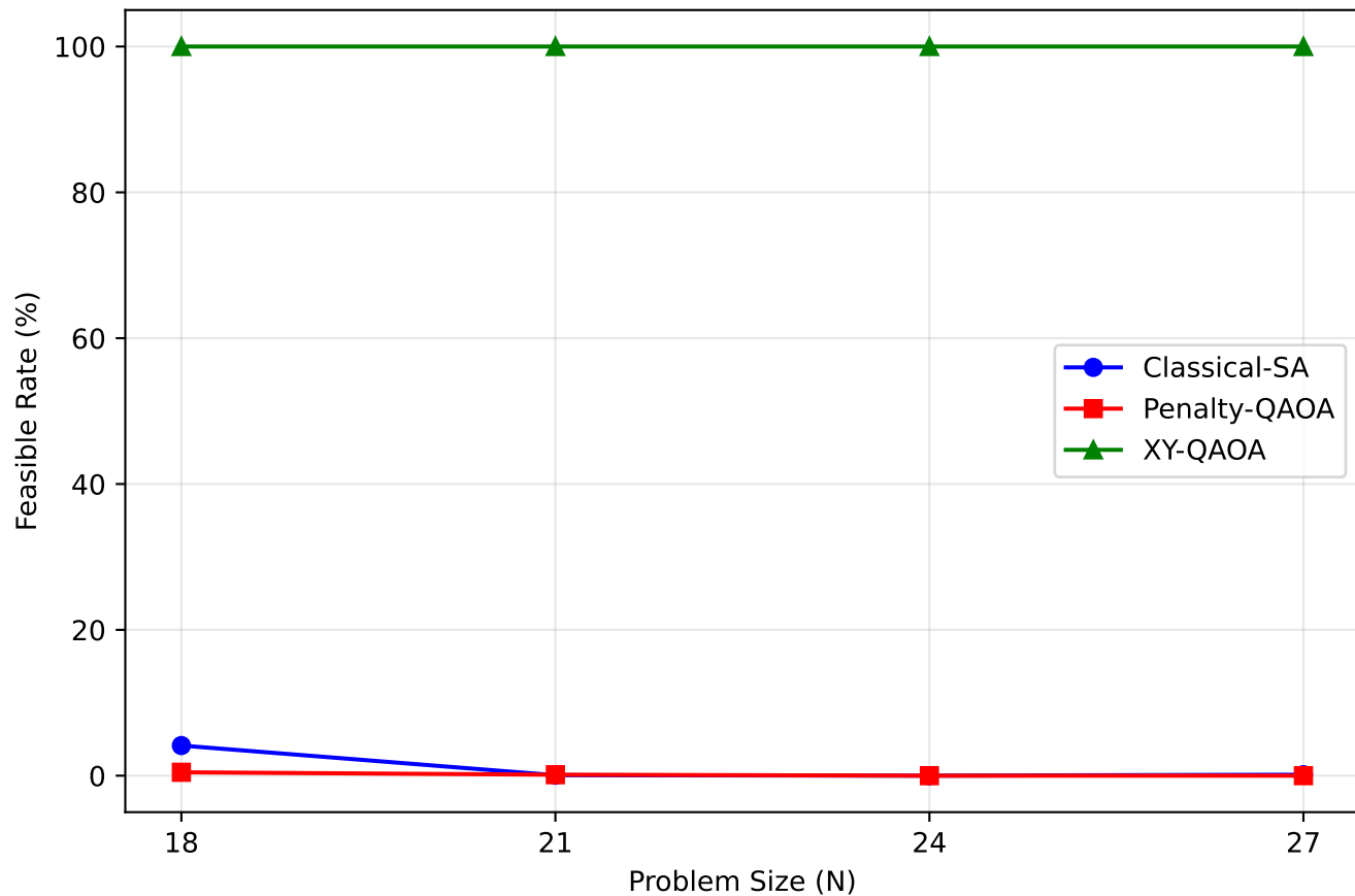
Feasible Rate vs N (BB2, Train N=200)
