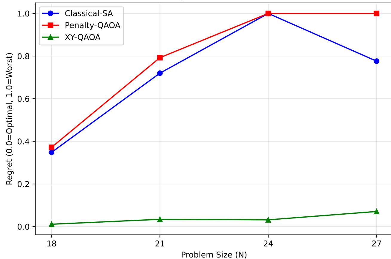
Normalized Regret vs N (BB2, Train N=200)
