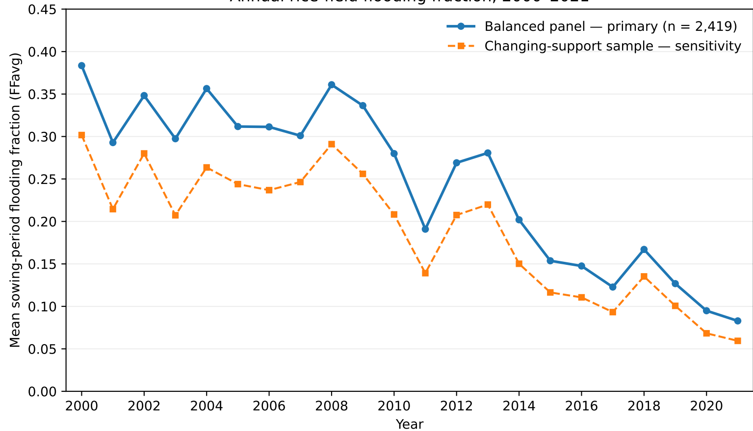
Annual rice-field flooding fraction, 2000-2021
