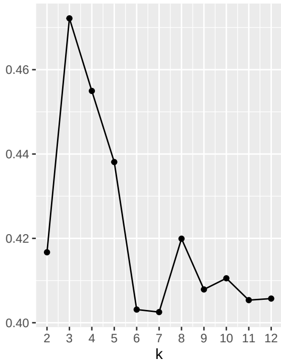
Mean silhouette width
