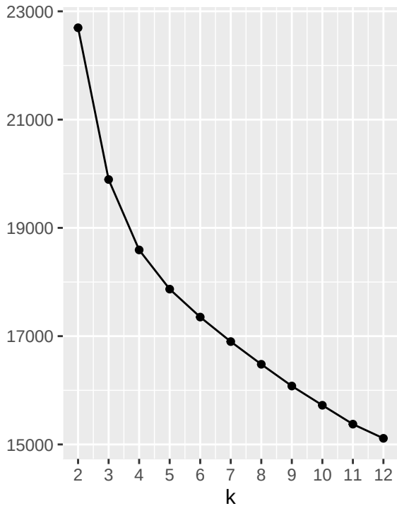
Within-cluster SS
