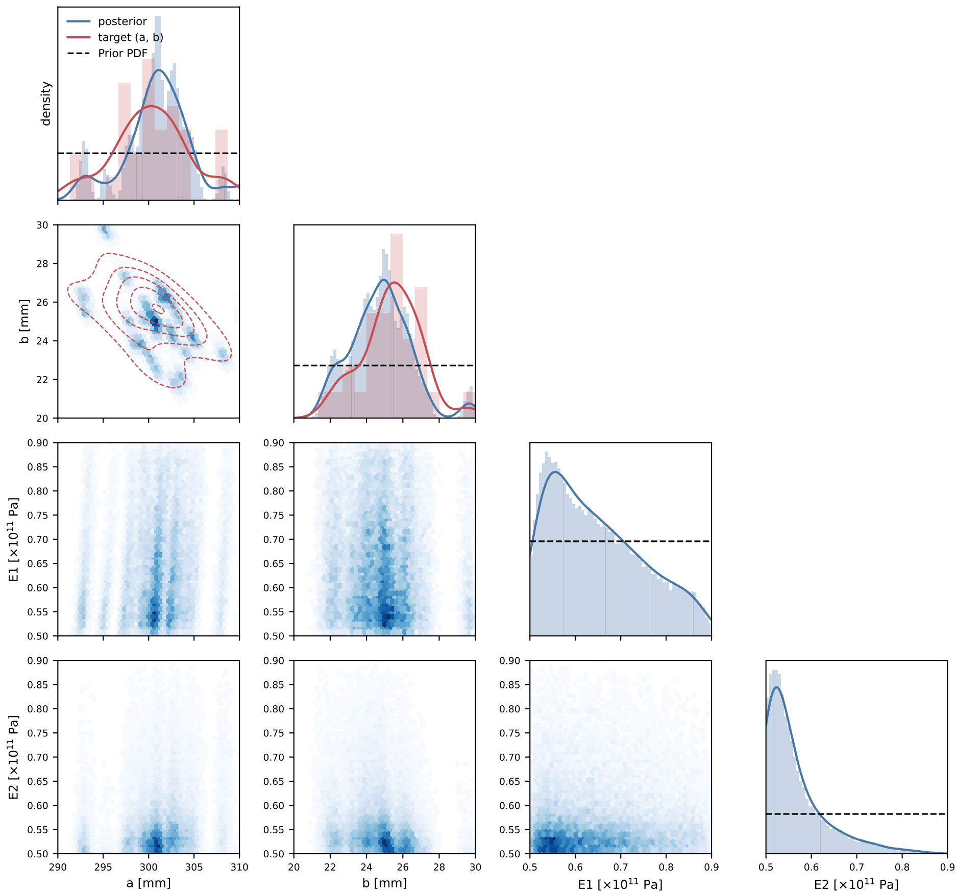
cFM | pooled posterior vs target (histogram + KDE)
