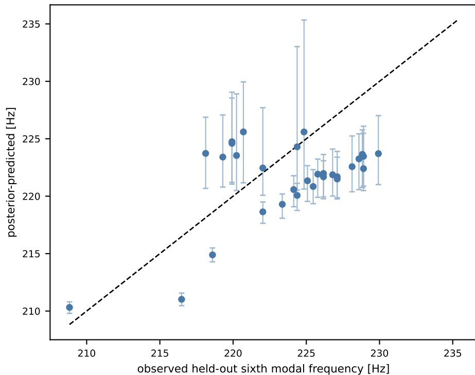
cVAE | posterior-predicted vs observed D_B=0.057 RMSE=4.49 bias=-2.19 cov=0.10
