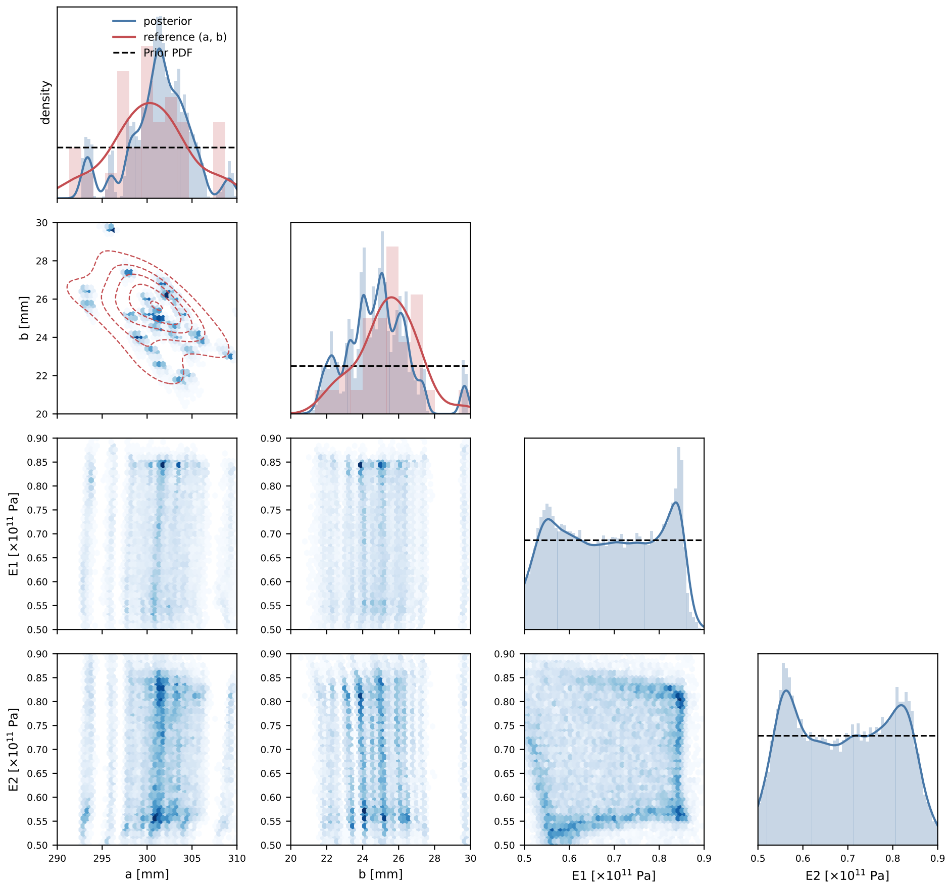
cGAN | pooled posterior vs reference (histogram + KDE)
