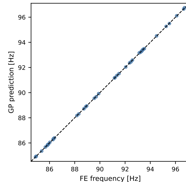
Mode 6 ( R^2=0.99985 )
