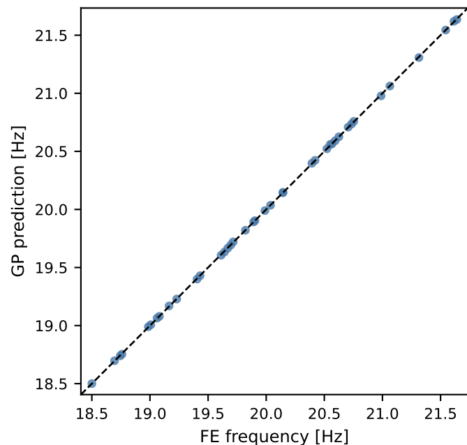
Mode 4 ( R^2=0.99997 )
