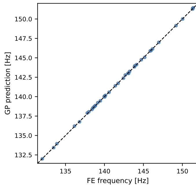
Mode 5 ( R^2=0.99989 )
