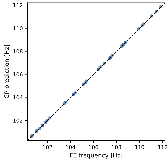
Mode 4 ( R^2=0.99997 )
