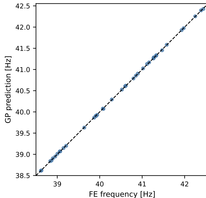
Mode 5 ( R^2=0.99989 )
