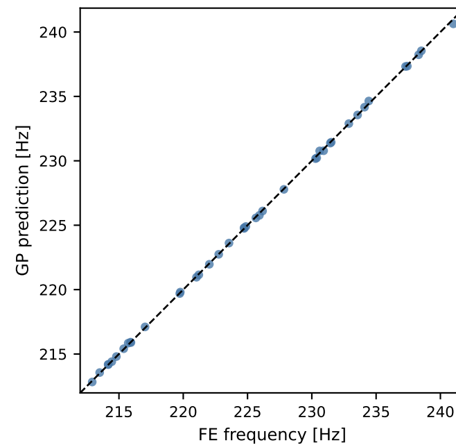
Mode 6 ( R^2=0.99985 )
