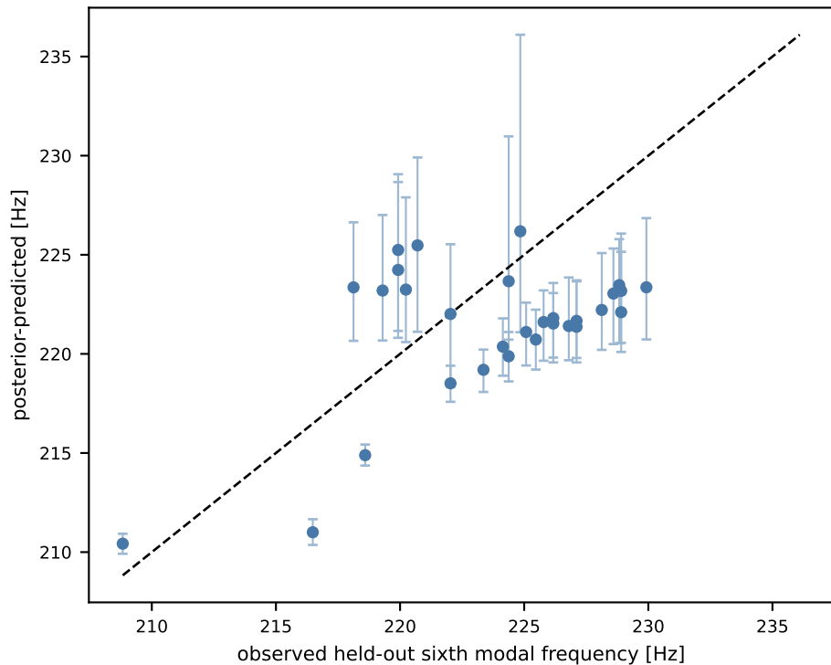
cNF | posterior-predicted vs observed D_B=0.063 RMSE=4.61 bias=-2.36 cov=0.10
