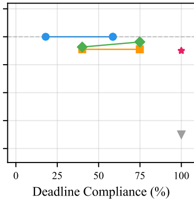
Qwen-14B
