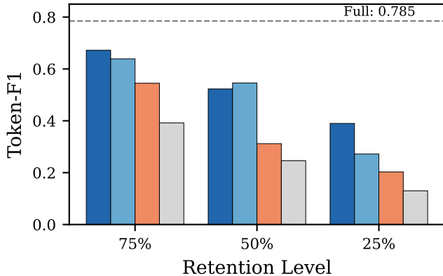
Qwen2.5-3B
