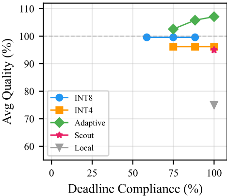
Qwen-7B
