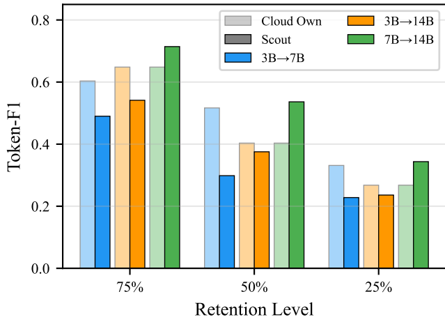
(b) F1: Cloud Own vs. Scout Selection
