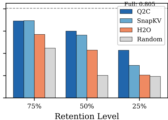
Qwen2.5-7B
