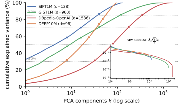
Figure 3: Cumulative explained variance on 100k samples, with components on a log scale. Each curve is a dataset’s prunability signature: by Eq. (3), the curve equals the expected fractional tightness of a width- k bound. Dots mark the widths the funnel selects at the {30, 50, 70, 85}% targets (dotted lines). SIFT and GIST have steep heads. DBpedia’s curve is shifted to the right, which is why a fixed d=128 ladder misreads it as unprunable. DEEP is the flattest, which matches its MODERATE verdict; its last width sits below the 85% line because of the d/2 cap. The inset shows the raw spectra (per-component variance fraction, log-log), for readers who want the decay rates directly.
