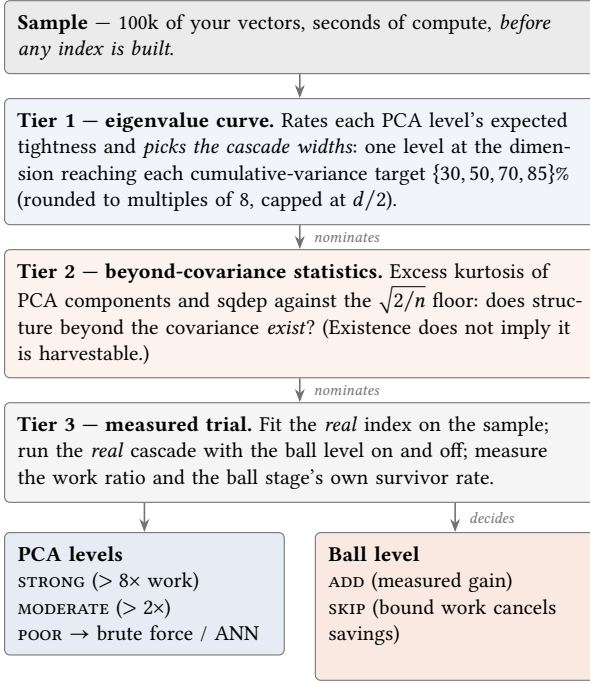
Figure 2: The self-configuration funnel. Tiers 1–2 are cheap statistics, and they may only nominate . Tier 1 also derives the cascade widths from the eigenvalue curve. Tier 3 is a measured trial of the real cascade, and it alone decides . Section 6.5 shows that the sample verdicts hold at 10^6 – 10^7 scale. The tier-2 mispredictions in the text (SIFT and latent-8, in opposite directions) are why no statistic can replace the trial.
