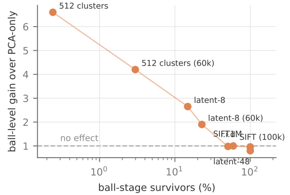
Figure 3: The measured ball-value law across all eight datasets and trials (parity code): the ball level’s wall-clock gain over the PCA-only cascade is a monotone function of its own pruning rate. The funnel’s tier-3 trial measures precisely the x -axis quantity, which is why it predicts full-scale outcomes from a sample—including the negative verdicts below the dashed line.
