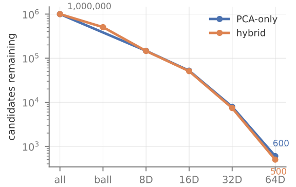
Figure 4: Candidates remaining after each stage on SIFT1M (log scale, average over 100 official queries). The cascade discards four orders of magnitude before any full-distance evaluation; the hybrid enters the PCA stages with half the population and finishes equally tight. This profile is the algorithmic fingerprint: it was invariant under every change of numeric type, machine load, and implementation tuning in this paper.
