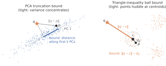
Figure 1: The two exact bound geometries. Left: the PCA truncation bound is the distance between the projections onto the first k principal components—tight when variance concentrates along few directions. Right: the ball bound \|q - c\| - d_p from the triangle inequality—tight when points huddle near their centroids. Each is loose exactly where the other is tight.
