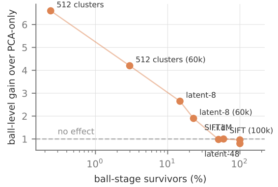
Figure 2: The measured ball-value law across all eight datasets and trials (parity code): the ball level’s wall-clock gain over the PCA-only cascade is a monotone function of its own pruning rate. The funnel’s tier-3 trial measures precisely the x -axis quantity, which is why it predicts full-scale outcomes from a sample—including the negative verdicts below the dashed line.
