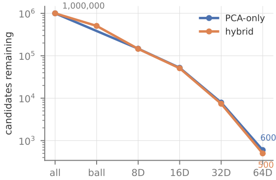
Figure 3: Candidates remaining after each stage on SIFT1M (log scale, average over 100 official queries). The cascade discards four orders of magnitude before any full-distance evaluation; the hybrid enters the PCA stages with half the population and finishes equally tight. This profile is the algorithmic fingerprint: it was invariant under every change of numeric type, machine load, and implementation tuning in this paper.
