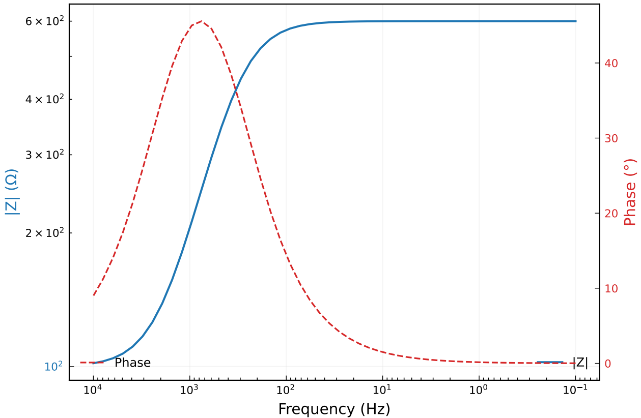
Bode Plot — acs-annotated
