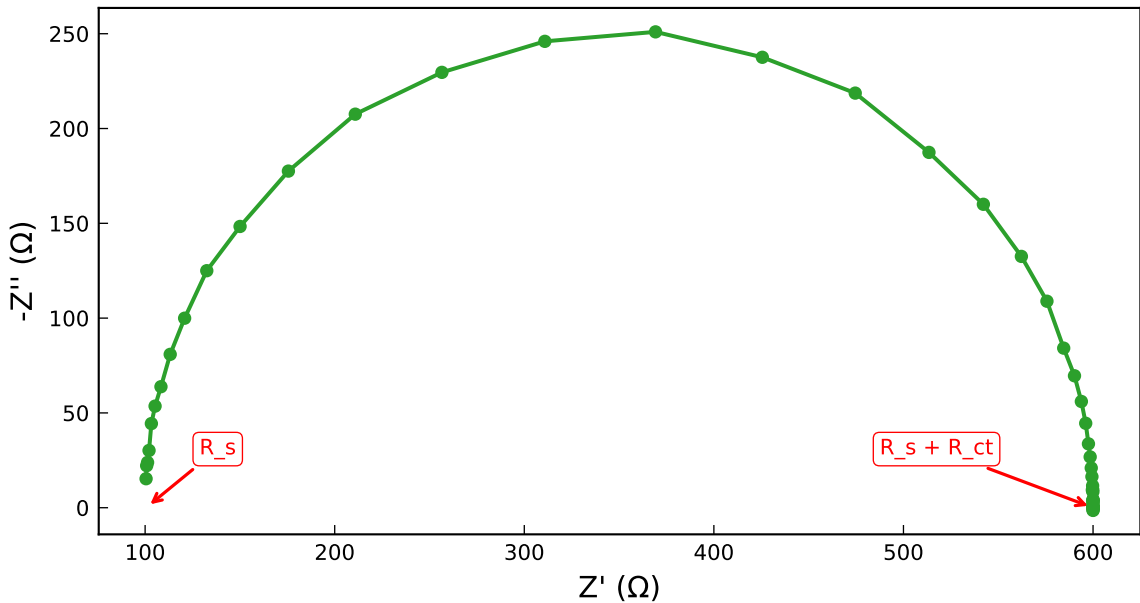
Nyquist Plot — acs-annotated
