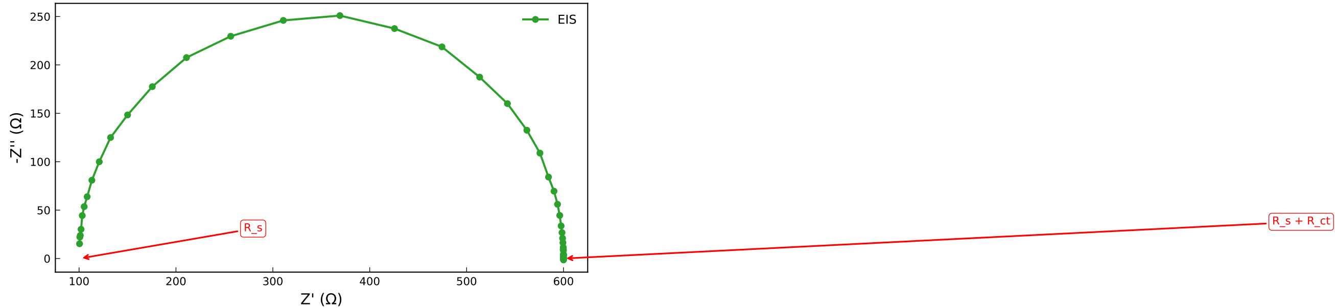
Nyquist Plot — acs-annotated
