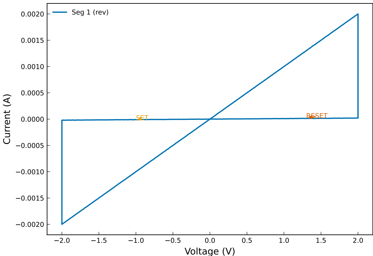
IV Curve — acs-annotated (annotated)
