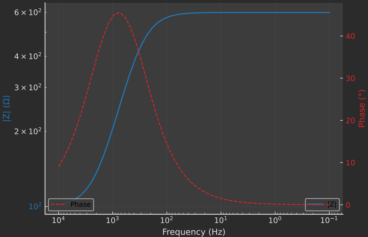
Bode Plot — dark
