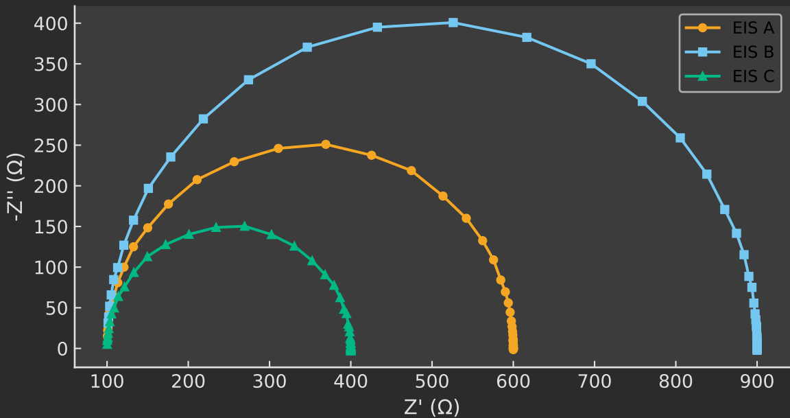
Nyquist Overlay — dark
