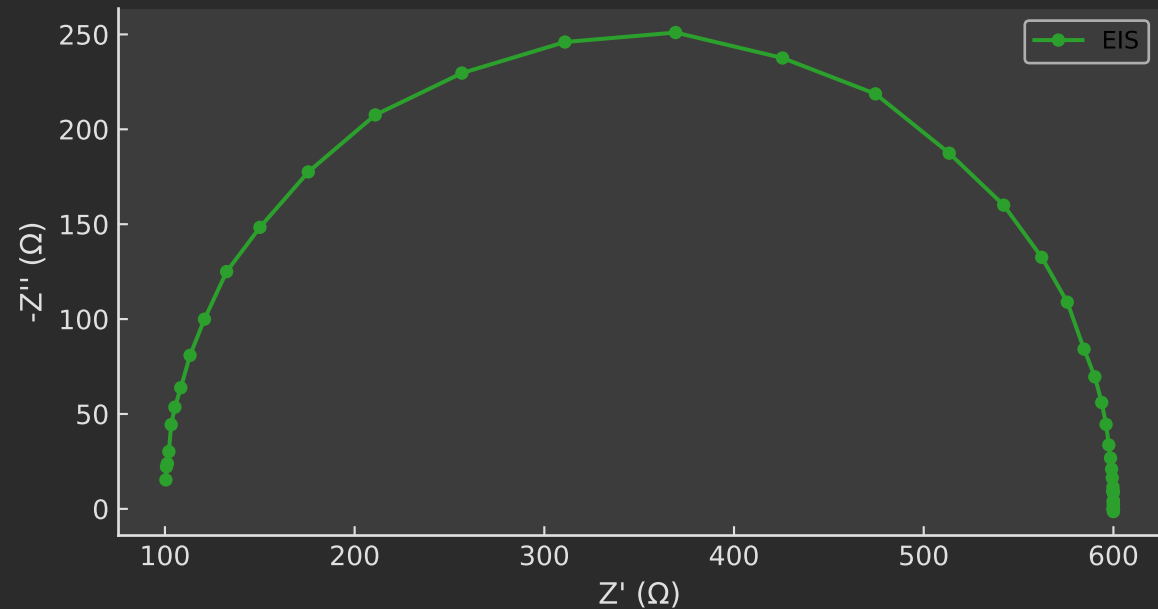
Nyquist Plot — dark
