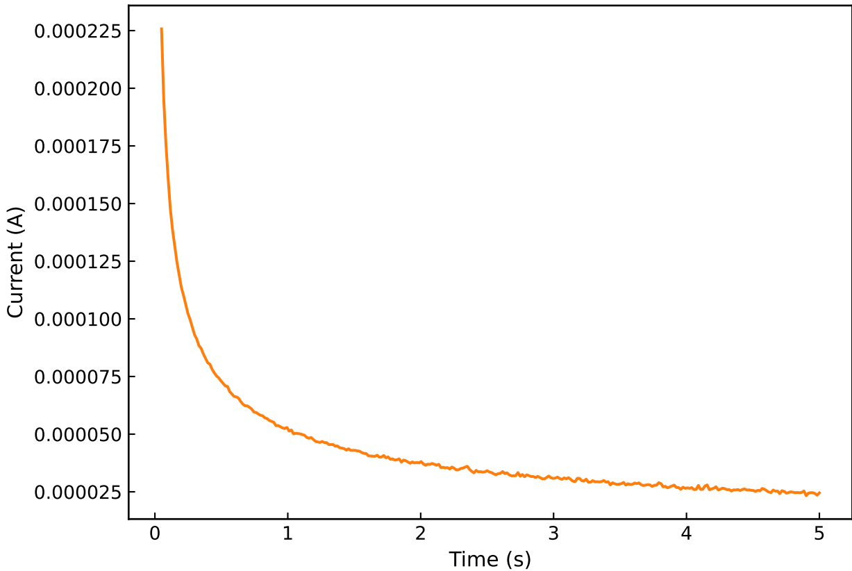
Chronoamperometry — default
