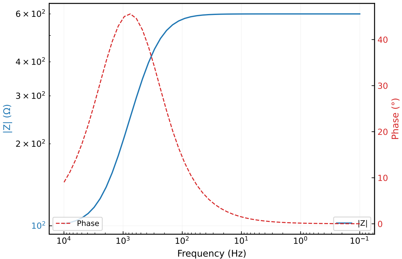
Bode Plot — default
